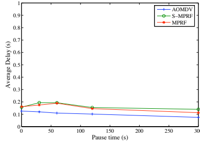
(b) Packet Delay
