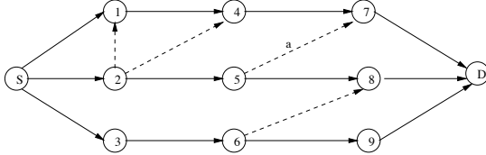
Fig. 2. Non-Disjoint Multi-Paths
